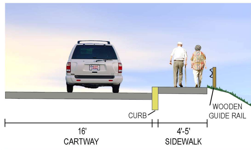
Typical Section of Chesterbrook Boulevard (South of 202 Looking North)
