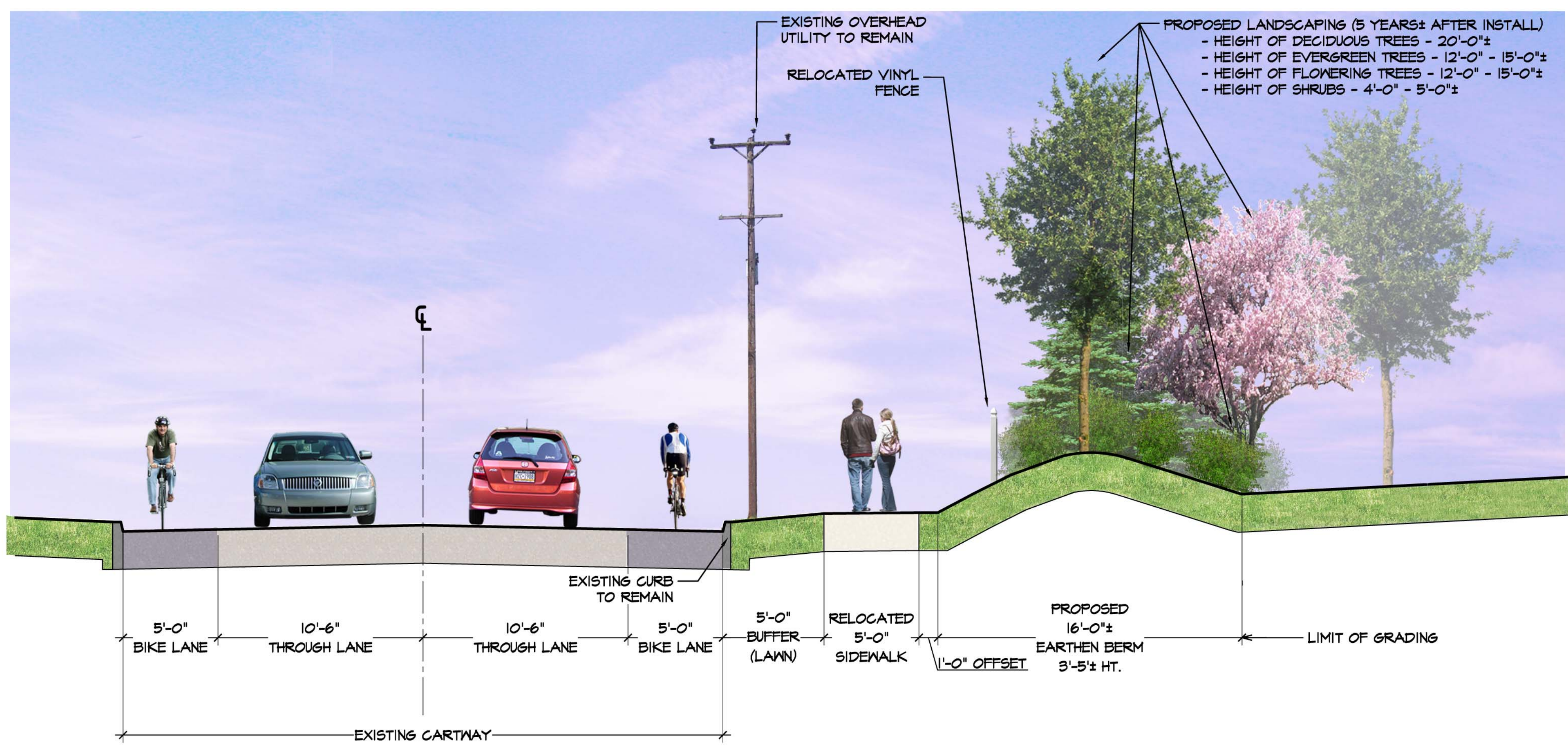
1 PROPOSED TYPICAL CENTRAL AVENUE SECTION SCALE 1/4"=1'-0"
